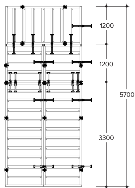
Formwork height: 5.70 m
