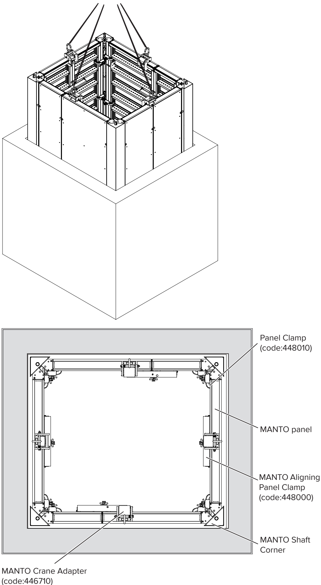
Example: Shaft formwork with MANTO Shaft Corners
