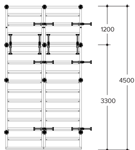
Formwork height: 4.50 m
