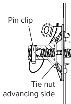
With pin clip inserted
