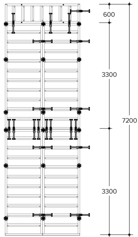
Formwork height: 7.20 m
