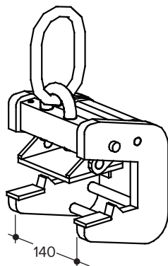
MANTO Crane Adapter (code:446710)
